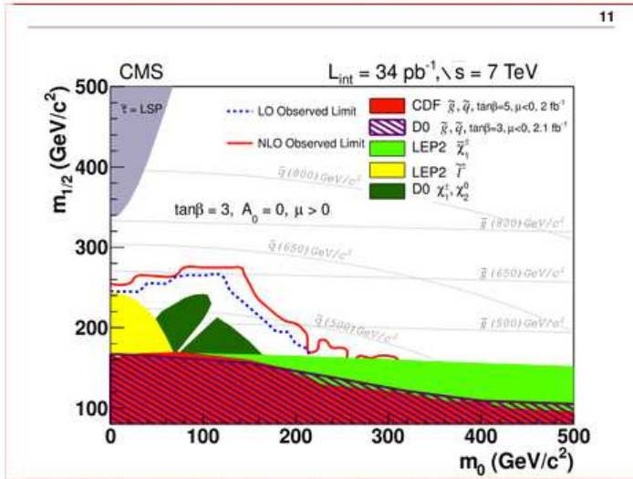
Figure 4: The observed 95% CL exclusion contour at NLO (solid red line) and LO (dashed blue line) in the CMSSM (m_0, m_{1/2}) plane for \tan\beta = 3 , A_0 = 0 and \mu > 0 . The area below the curve is excluded by this measurement. Exclusion limits obtained from previous experiments are presented as filled areas in the plot. Thin grey lines correspond to constant squark and gluino masses.
