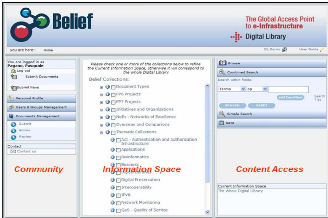
Figure 1 – The DL Desktop organization
